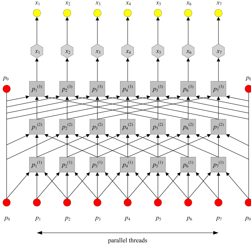
Figure 2: Routing diagram of the parallel cyclic reduction algorithm. The symbols have the same meaning as in figure 1.
